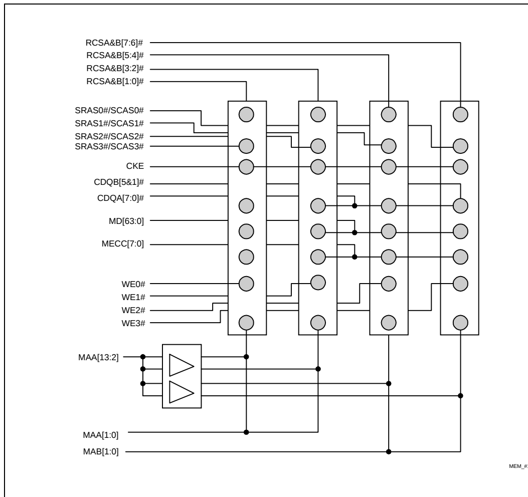
Figure 5. Configuration #1 (Large Memory Array)
