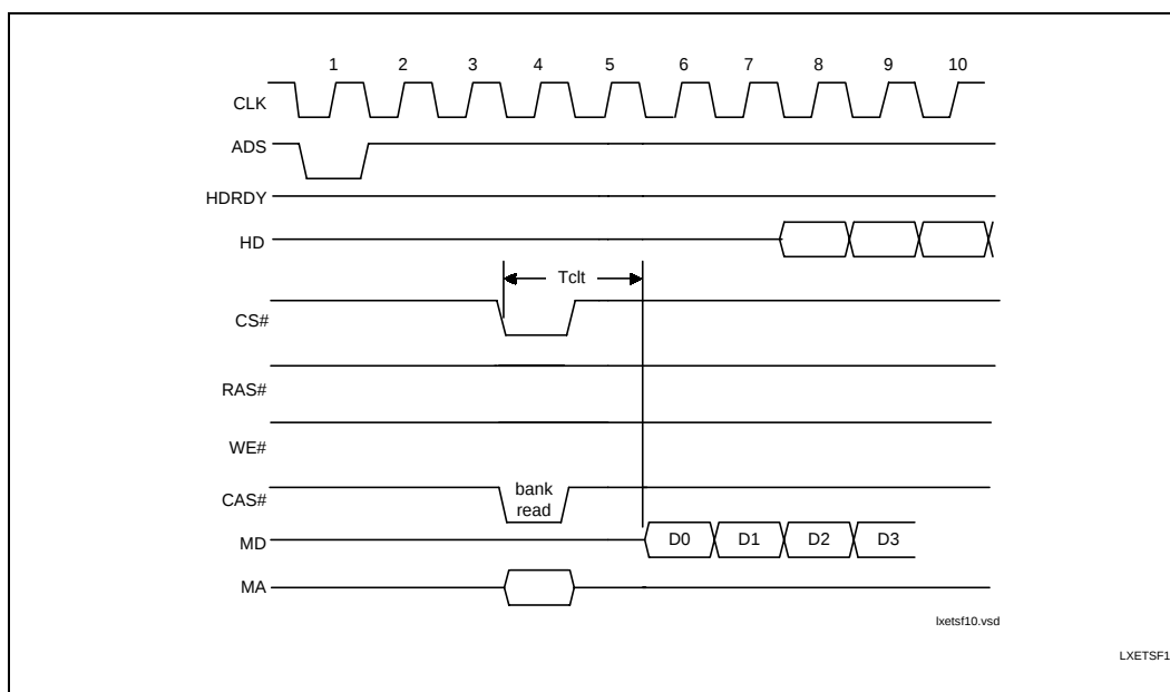
Figure 24. Page Hit with SCLT=1, SRCD=1, SRPT=1
