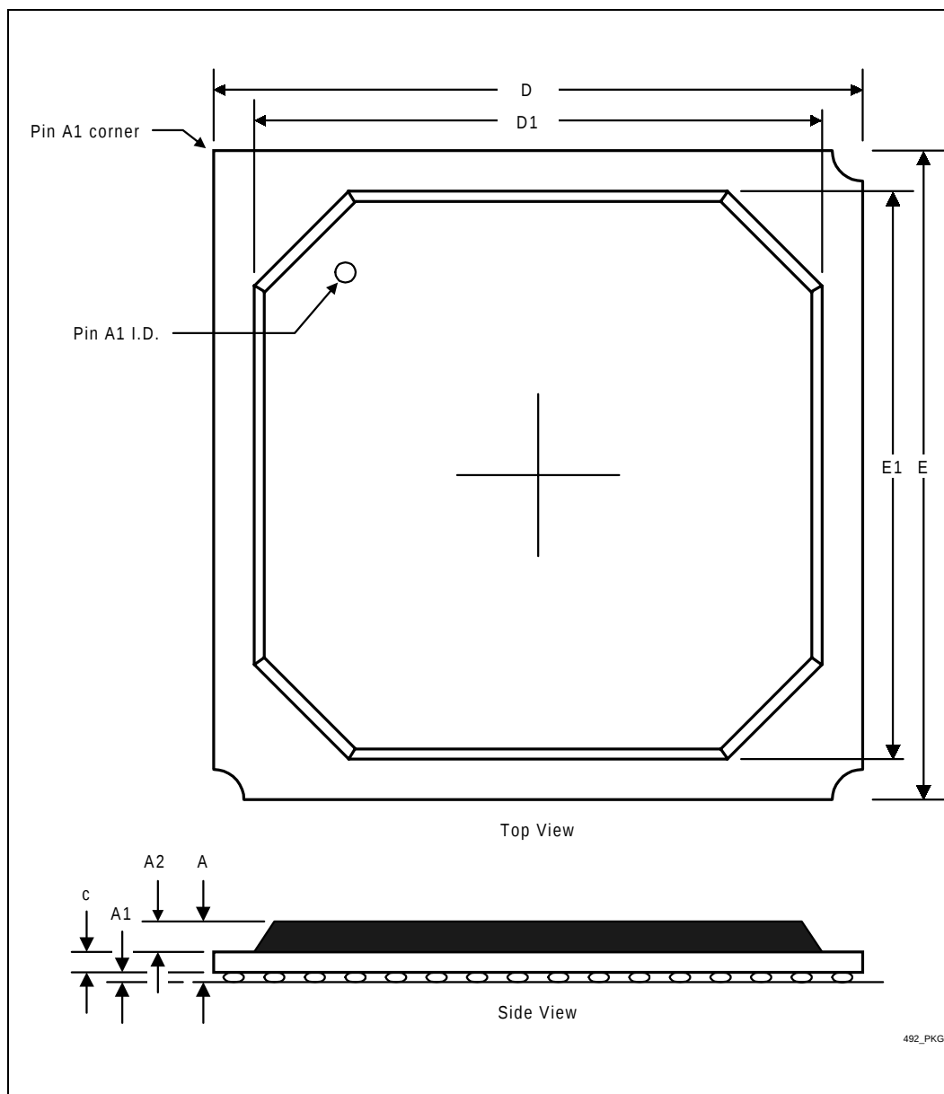
Figure 34. PAC Package Dimensions (492 BGA)
