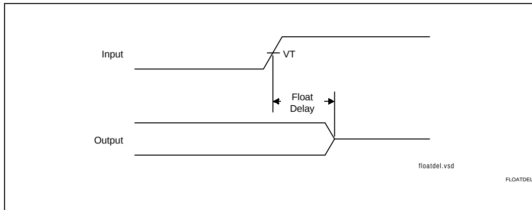
Figure 19. Float Delay
