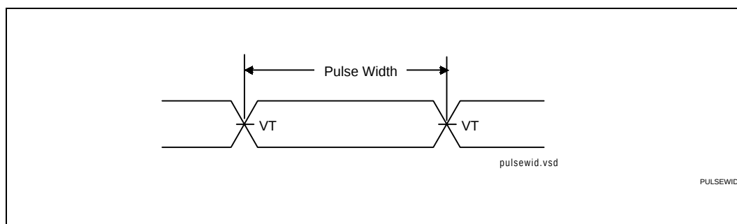
Figure 20. Pulse Width
