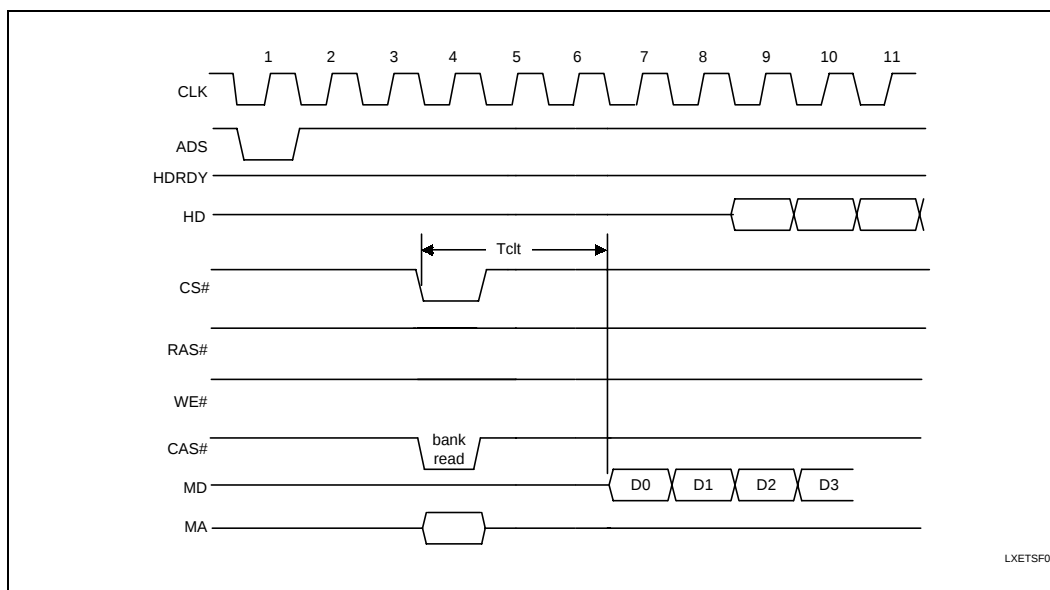
Figure 23. Page Hit with SCLT=0, SRCD=1, SRPT=1
