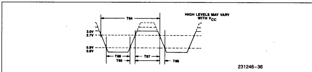
Figure 35. RxC Input Voltage Levels for Timing Measurements *
