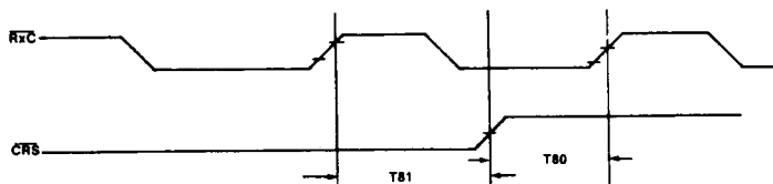
Figure 38. \overline{CRS} Timing Relative to \overline{Rx}C
