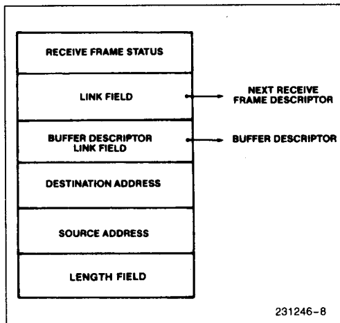
Figure 9. Receive Frame Descriptor
