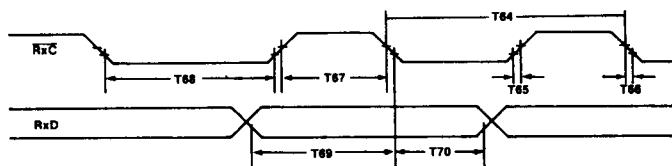
Figure 37. \overline{Rx}D Timing Relative to \overline{Rx}C
