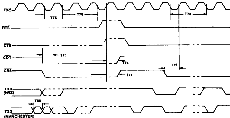
Figure 36. Transmit and Control and Data Timing
