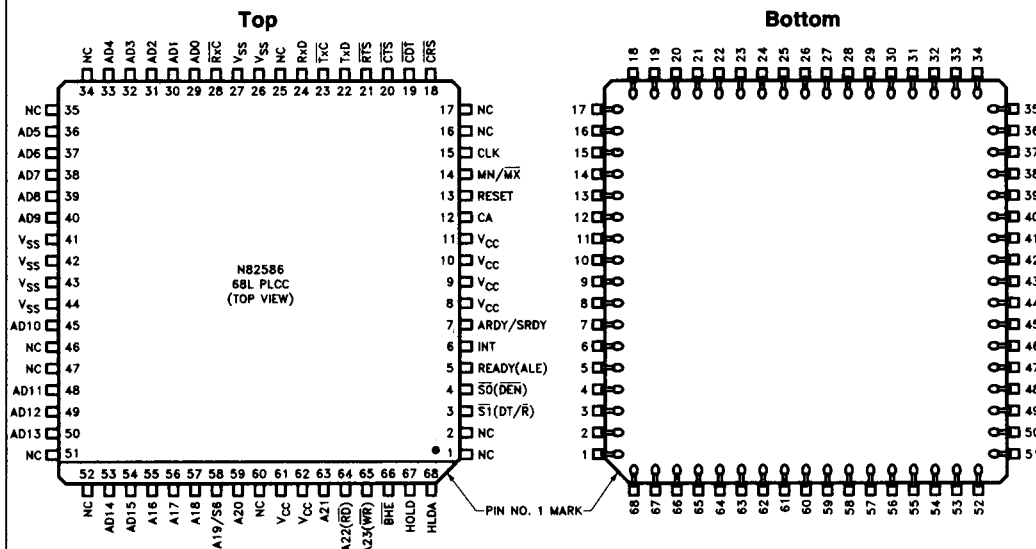
Figure 2. 82586 Pinout Diagrams
