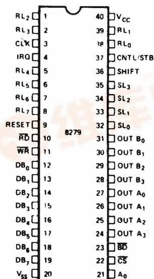
Figure 2. Pin Configuration
