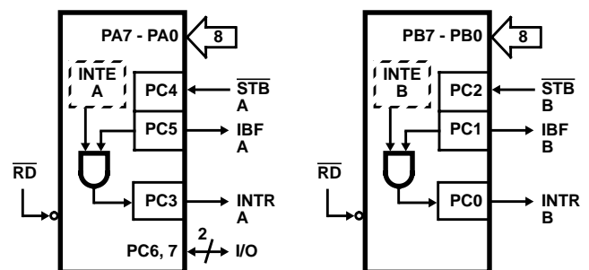
FIGURE 15. MODE 1 INPUT
