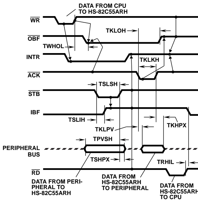
FIGURE 5. MODE 2 (BIDIRECTIONAL)
