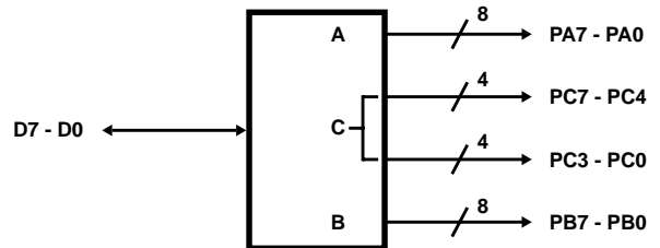
CONTROL WORD #11
