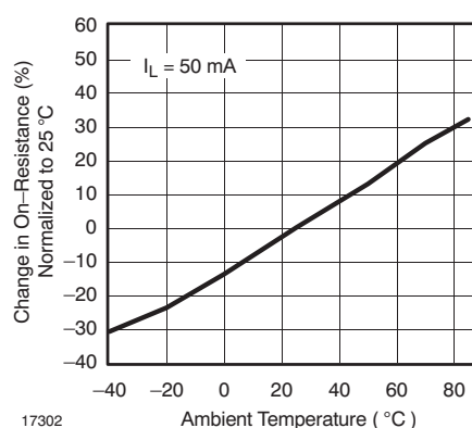
Figure 3. ON-Resistance vs. Temperature
