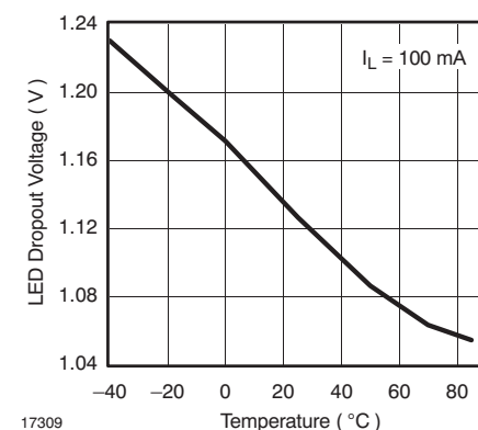
Figure 10. LED Dropout Voltage vs. Temperature
