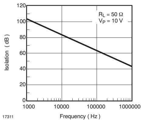
Figure 12. Output Isolation
