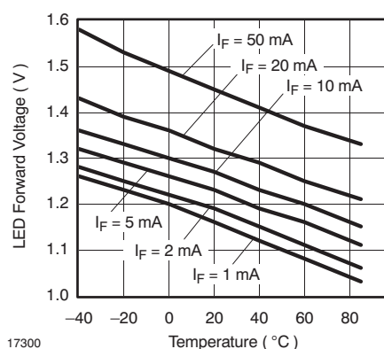
Figure 1. LED Voltage vs. Temperature
