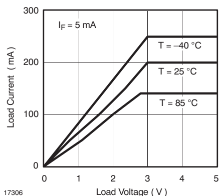
Figure 7. Load Current vs. Load Voltage
