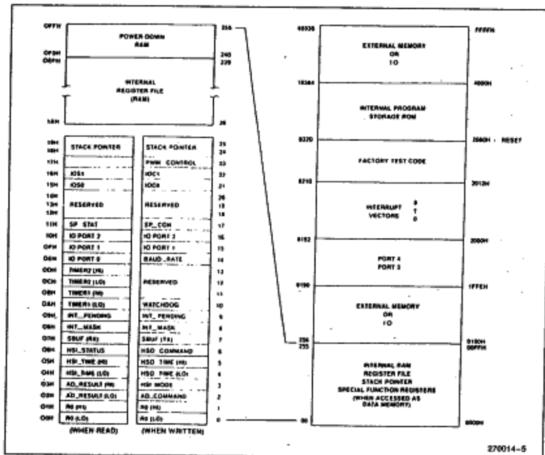
Figure 5. Memory Map
