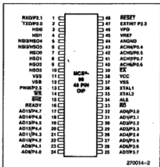
Figure 2. 48-Pin Package
