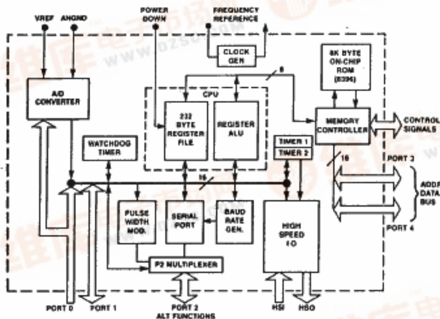
Figure 1. Block Diagram
