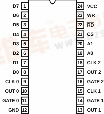
82C54 (PDIP, Cerdip, SOIC) TOP VIEW
