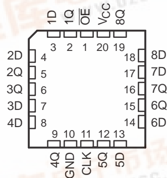
SN54HCT374 ... FK PACKAGE (TOP VIEW)
