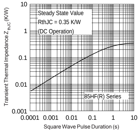
Fig. 13 - Thermal Impedance Z_{thJC} Characteristics
