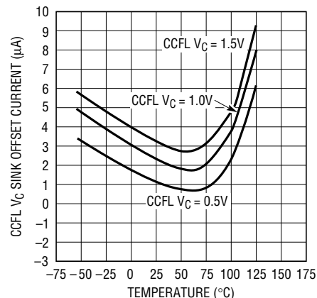
V_C Sink Offset Current vs Temperature
