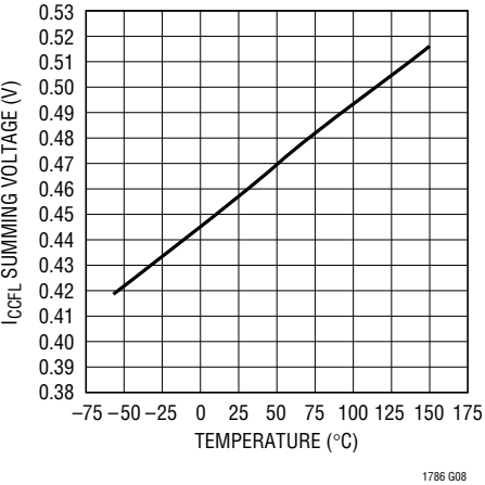
I CCFL Summing Voltage vs Temperature
