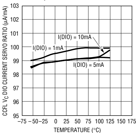
V_C to DIO Current Servo Ratio vs Temperature
