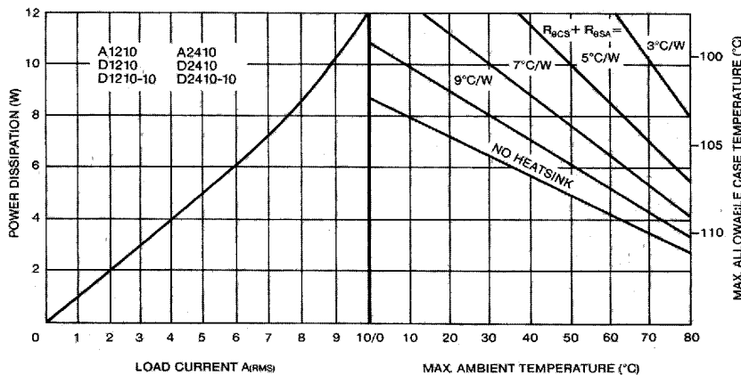
Figure 5. Thermal Derating Curves: 10 Amp, 120 and 240V.
