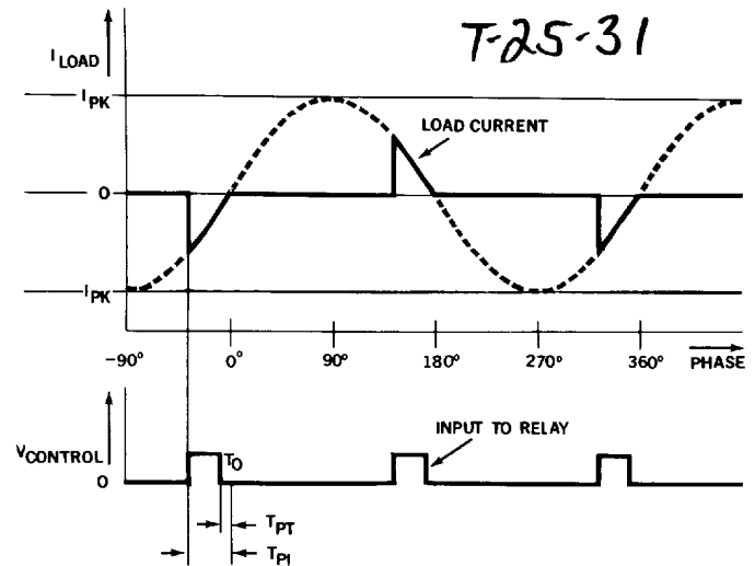
Figure 10 The relationship of zero current time, pulse termination time, and pulse initiation time to load current time
