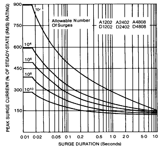
Figure A. Peak Surge Current vs. Duration: 2 and 8 Amp Models.
