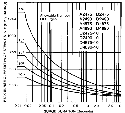
Figure E. Peak Surge current vs. Duration: 75 &amp; 90 Amp Models.
