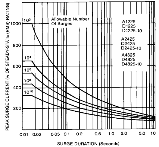
Figure C. Peak Surge Current vs. Duration: 25 Amp Models.
