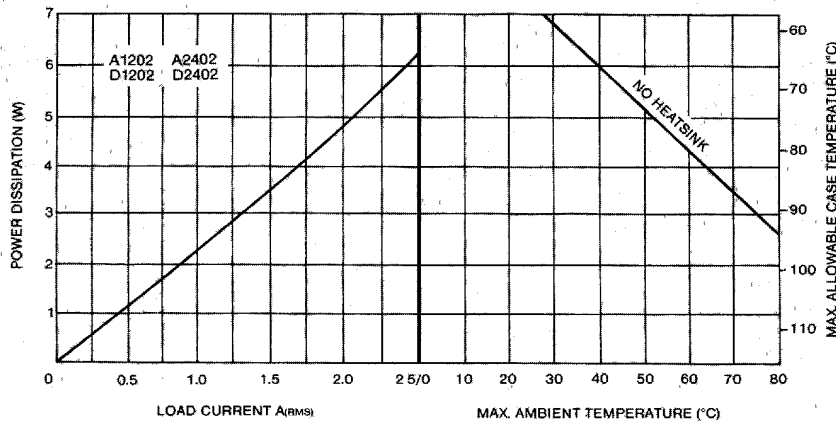
Figure 4. Thermal Derating Curves: 2.5 Amp, 120 and 240V.
