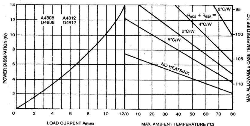
Figure 6. Thermal Derating Curves: 8 and 12 Amp, 480V.
