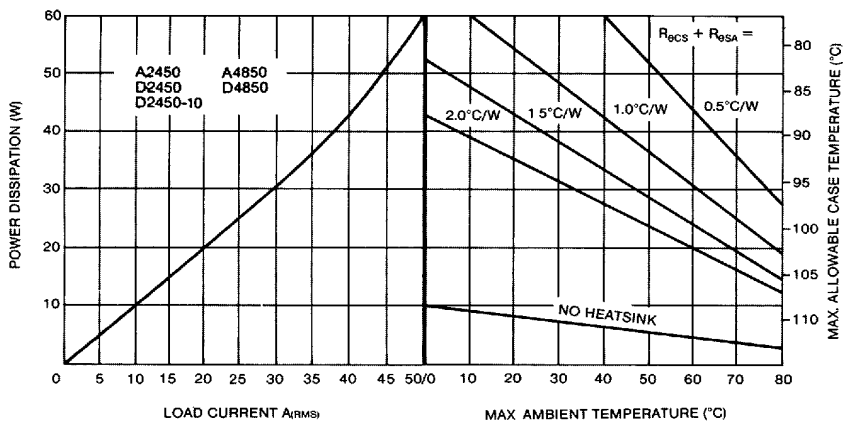
Figure 8. Thermal Derating Curves: 50 Amp, 240 V.
