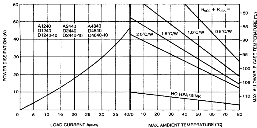
Figure 7. Thermal Derating Curves: 40 Amp, 120/240 and 480V.
