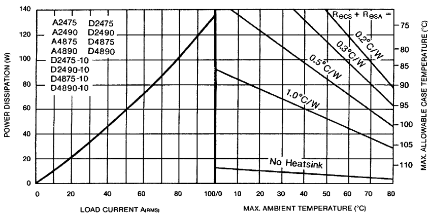
Figure 9. Thermal Derating Curves 75 &amp; 90 Amp., 240 and 480V.
