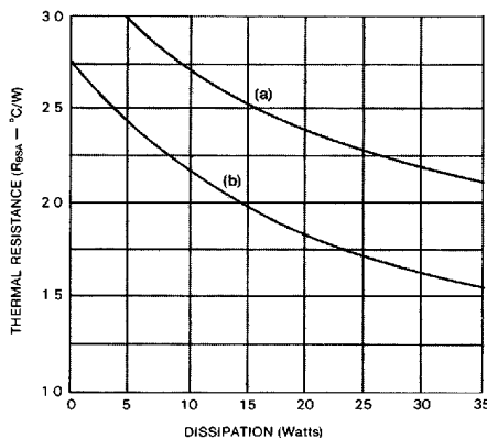
Figure 2. Typical Heat Sink Characteristics See Page 7
