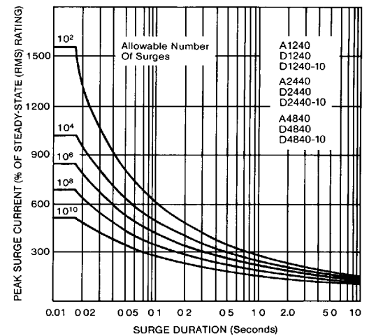
Figure D. Peak Surge Current vs. Duration: 40 Amp Models.
