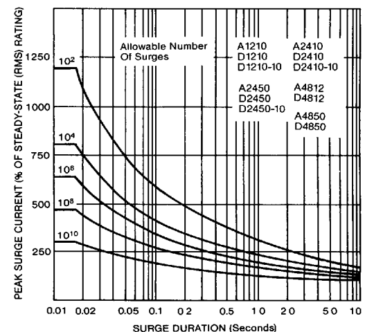
Figure B. Peak Surge Current vs. Duration: 10, 12 and 50 Amp Models.
