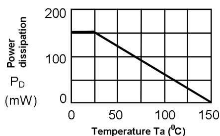
Figure 10 Power dissipation of an SOT-23-5 Package (Free-Air)
