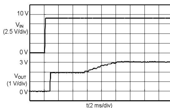
S-8520/1C30MC ( V_{IN} : 0 \rightarrow 9.0 V)
