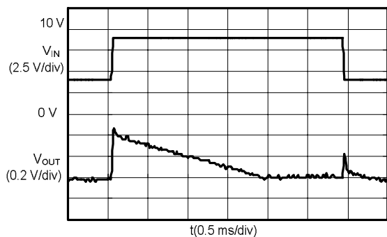
S-8520/1C33MC ( I_{OUT} :10 mA)
