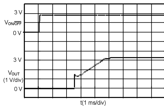
S-8520/1E33MC ( V_{IN} :9.0 V)
