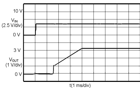
S-8520/1E33MC ( V_{IN} : 0 \rightarrow 4.0 V)
