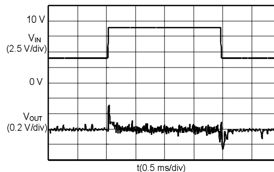
S-8520/1A30MC ( I_{OUT} :500 mA)
