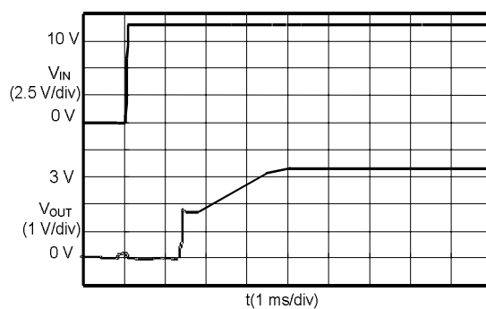
S-8520/1E33MC ( V_{IN} : 0 \rightarrow 9.0 V)
