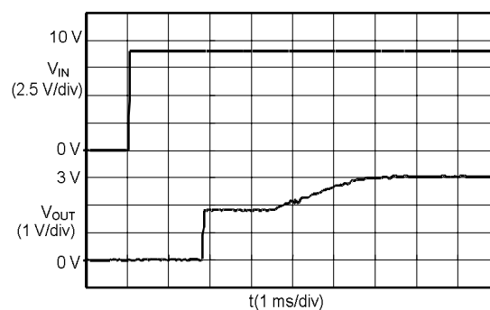
S-8520/1A30MC ( V_{IN} : 0 \rightarrow 9.0 V)
