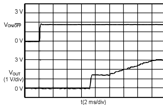
S-8520/1C30MC ( V_{IN} :9.0 V)
