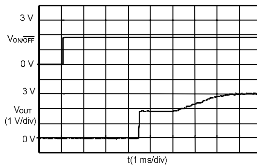
S-8520/1A30MC ( V_{IN} :9.0 V)
