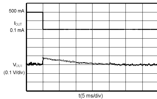
S-8520/1E33MC ( V_{IN} : 4.0 V)
