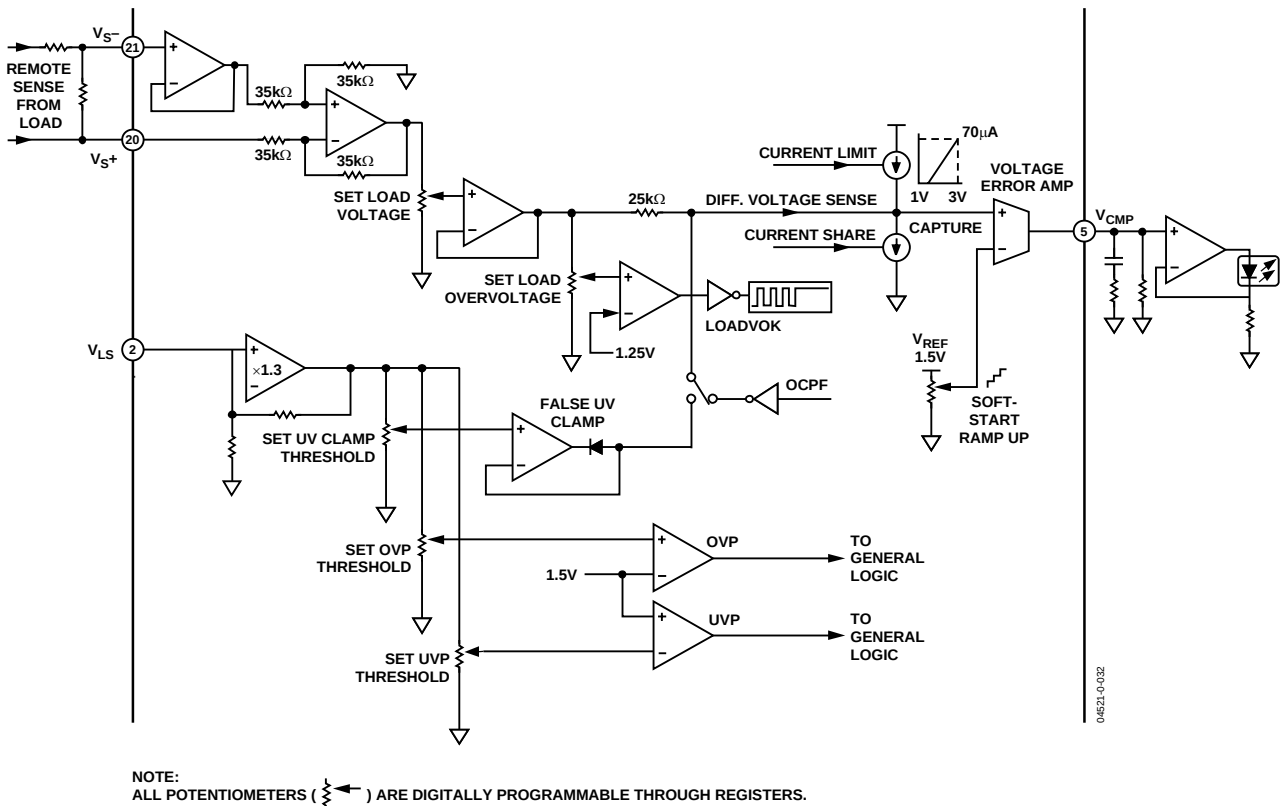
Figure 9. Block Diagram of Voltage Sense Amplifier
