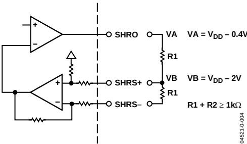
Figure 6. Amplifier Inputs and Outputs
