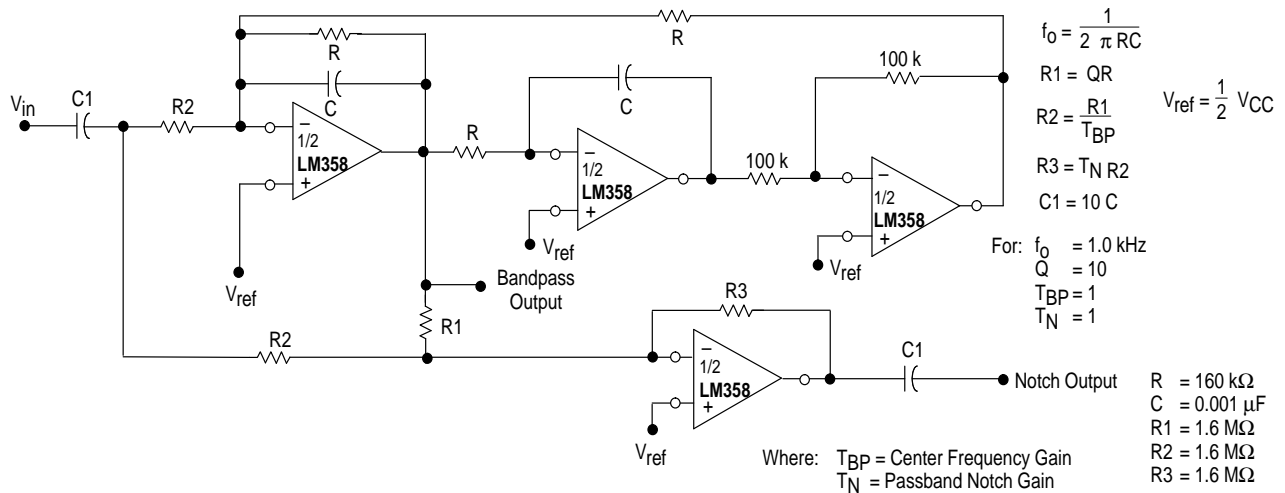
Figure 11. Bi-Quad Filter
