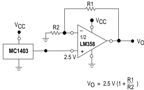
Figure 7. Voltage Reference
