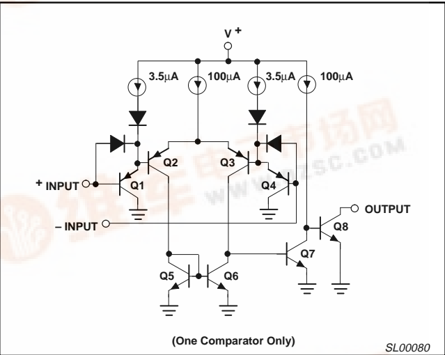
Figure 2. Equivalent Circuit
