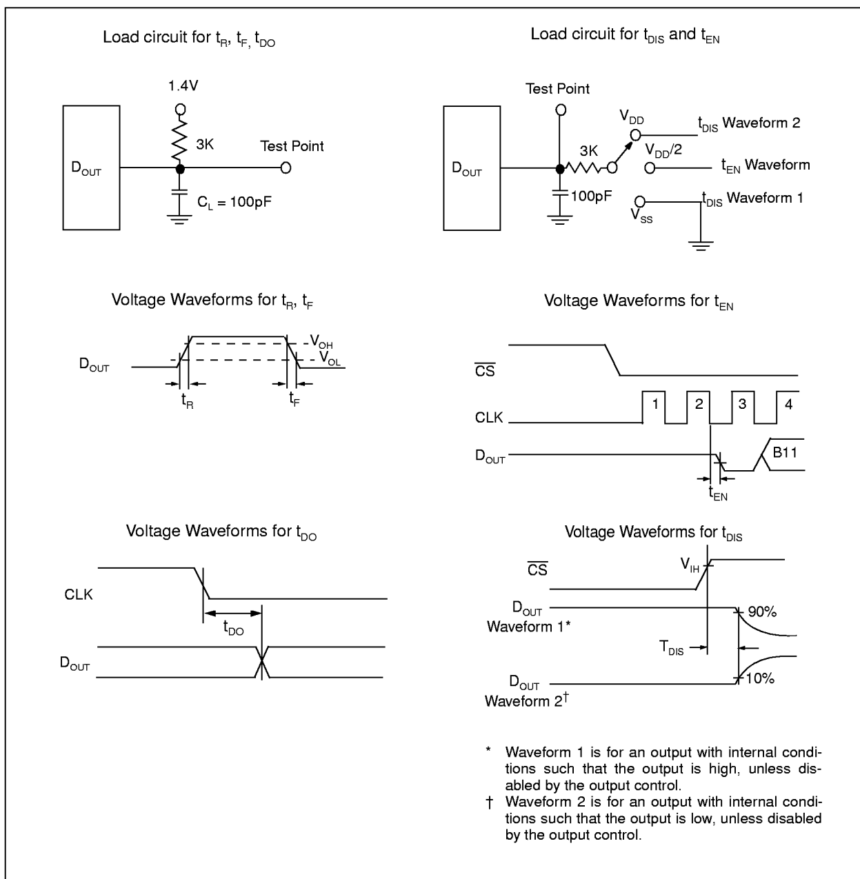
FIGURE 1-2: Test Circuits.
