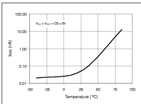
FIGURE 2-38: I_{DDs} vs. Temperature.
