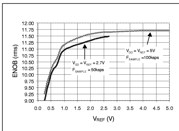
FIGURE 2-25: Effective Number of Bits (ENOB) vs. V_{REF} .
