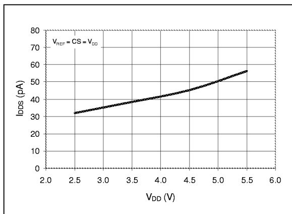
FIGURE 2-37: I_{DDs} vs. V_{DD} .
