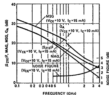
Figure 4. Typical |S_{21}|^2 , MAG, MSG, Noise Figure, and G , vs. Frequency, for the HSMX-3151.
