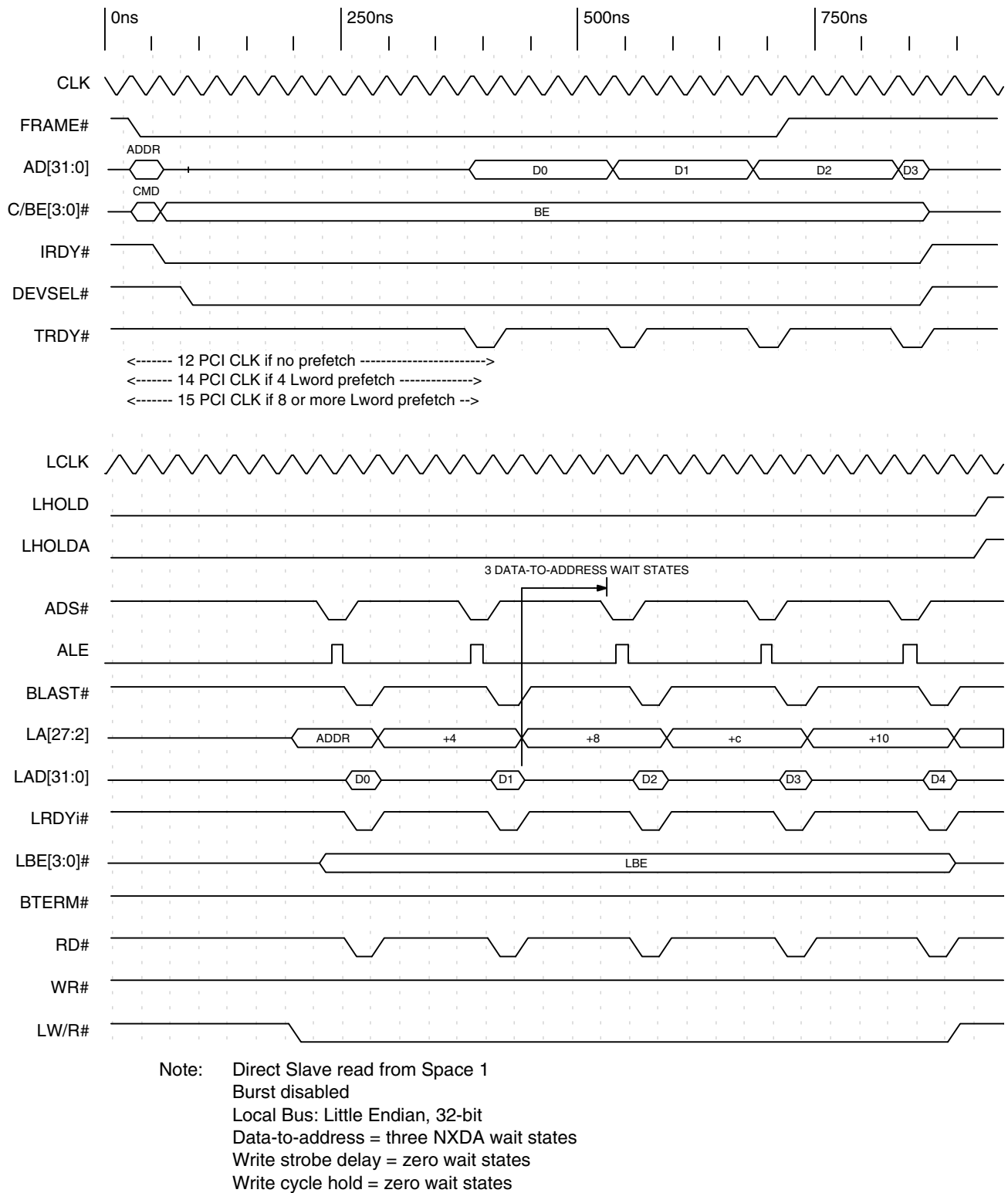
Timing Diagram 4-18. Non-Multiplexed Mode, Direct Slave Non-Burst Read (32-Bit Local Bus)
