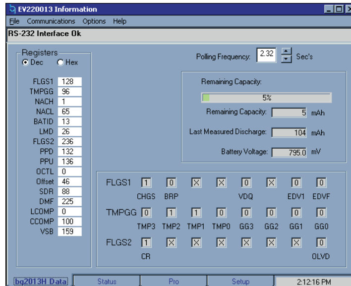
Figure 3. bq2013H Data Screen
