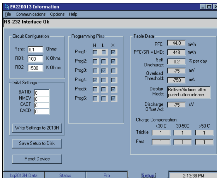
Figure 2. Setup Data Screen
