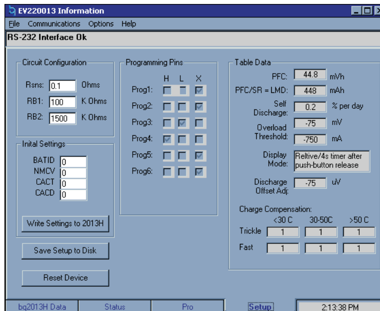
Figure 7. bq2013h Data Screen–Communication Failure
