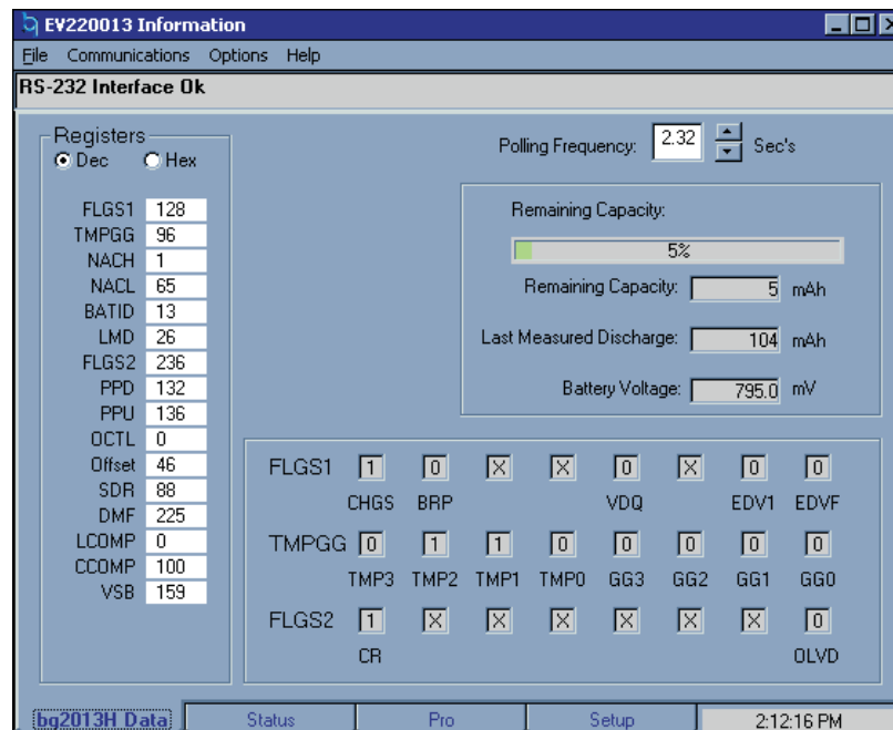
Figure 1. bq2013h Data Screen
