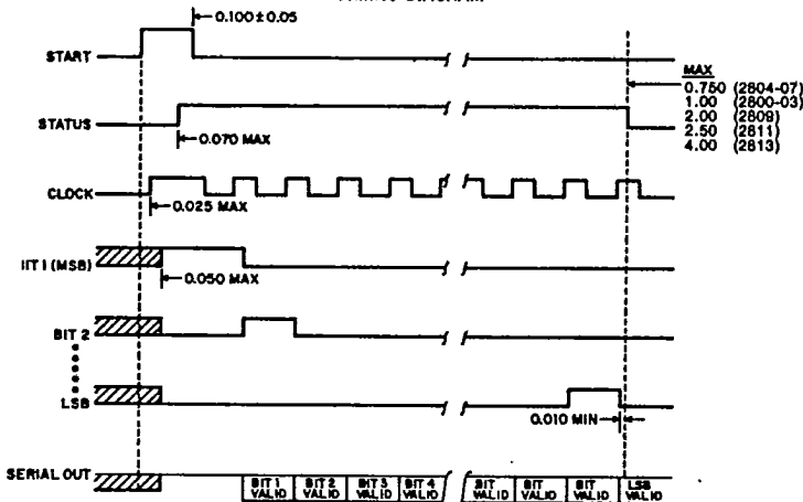
TIMING DIAGRAM
