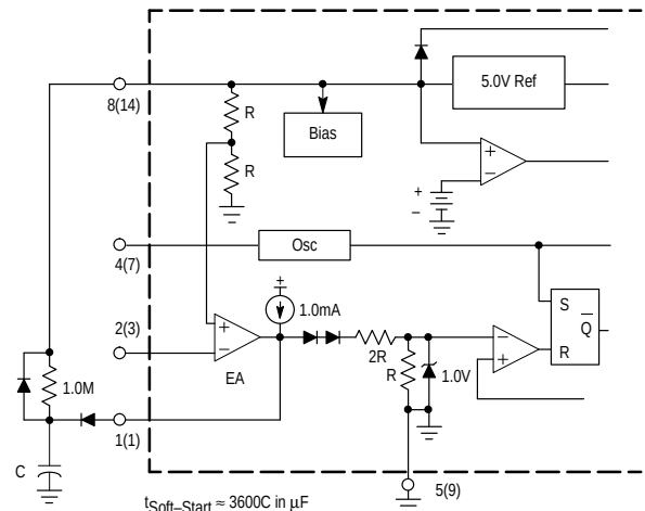
Figure 23. Soft-Start Circuit
