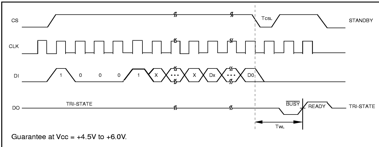
FIGURE 3-8: WRAL TIMING
