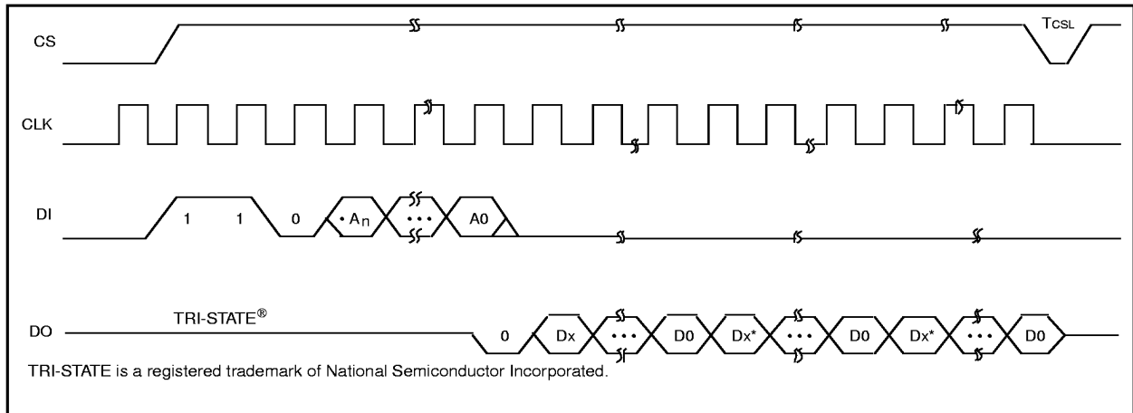
FIGURE 3-6: READ TIMING
