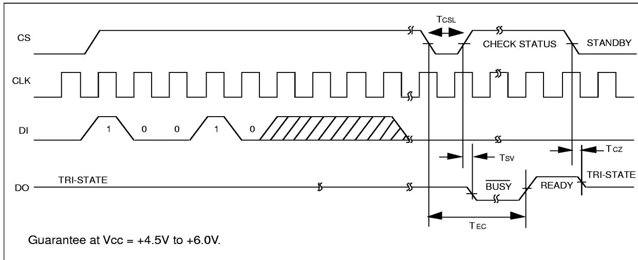
FIGURE 3-3: ERAL TIMING
