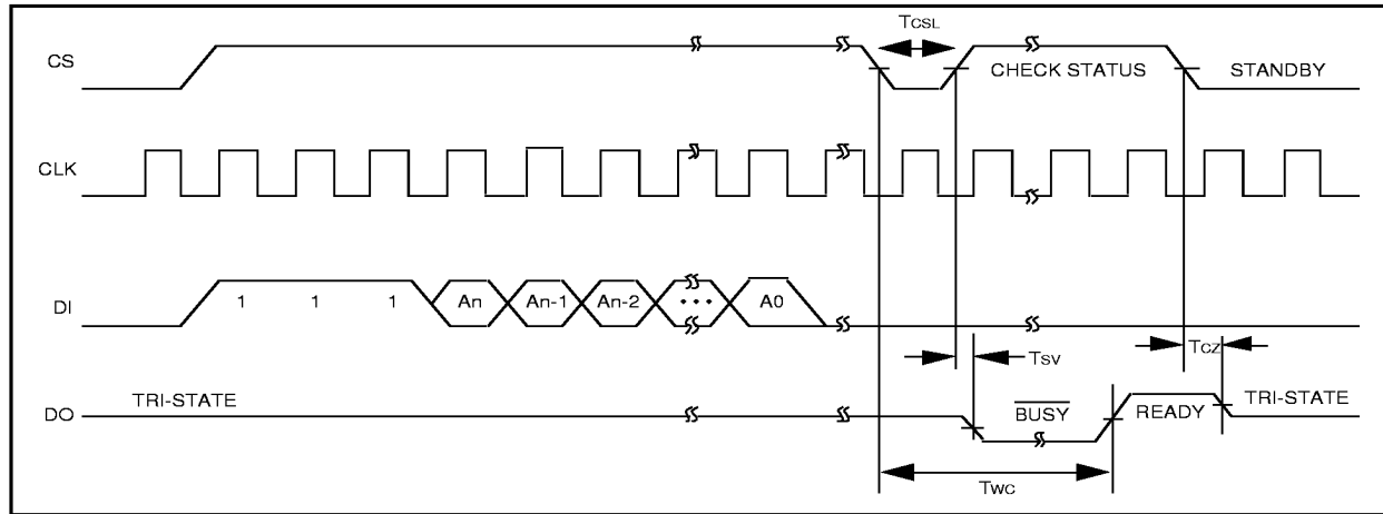
FIGURE 3-2: ERASE TIMING
