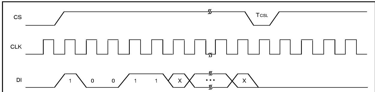
FIGURE 3-5: EWEN TIMING
