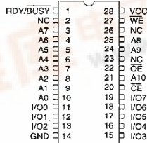
CERDIP, PDIP, SOIC Top View
