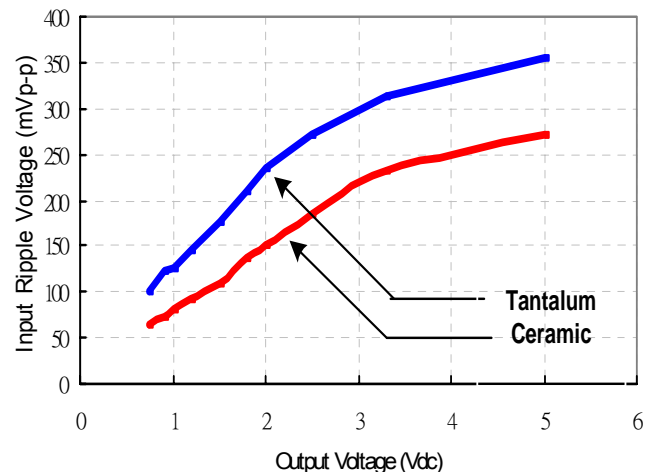
Figure 28: Input ripple voltage for various output models, I_o = 4A ( C_{in} = 2x47uF tantalum capacitors or 2x22uF ceramic capacitors at the input)
