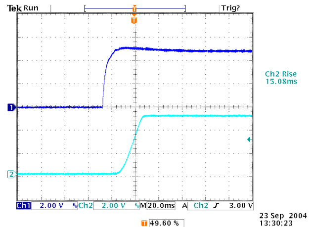
Figure 20: Remote turn on delay time at 12vin, 5.0V/4A out
