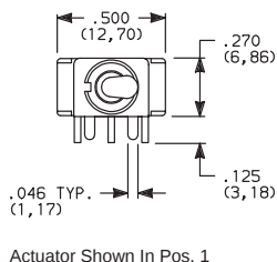
7101MD9A4BE Horizontal Actuation SPDT
