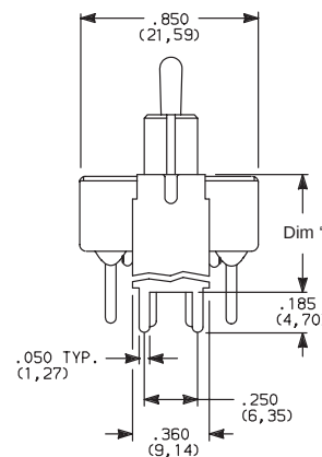
Snap-In
