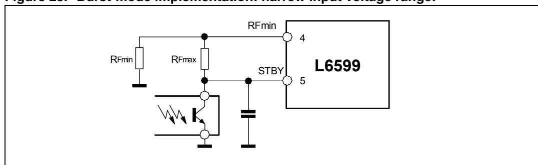
Figure 23. Burst-mode implementation: narrow input voltage range.
