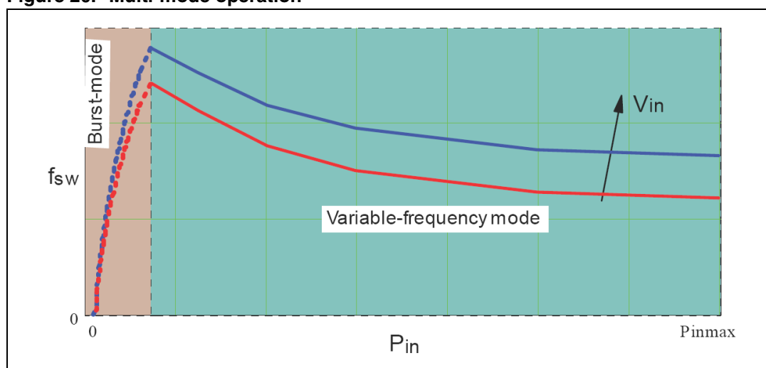
Figure 20. Multi-mode operation
