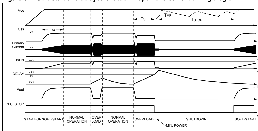
Figure 31. Soft-start and delayed shutdown upon overcurrent timing diagram
