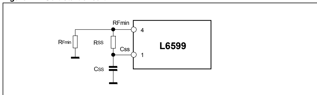
Figure 27. Soft-start circuit
