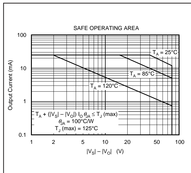
FIGURE 3. 8-Pin DIP Safe Operating Area.
