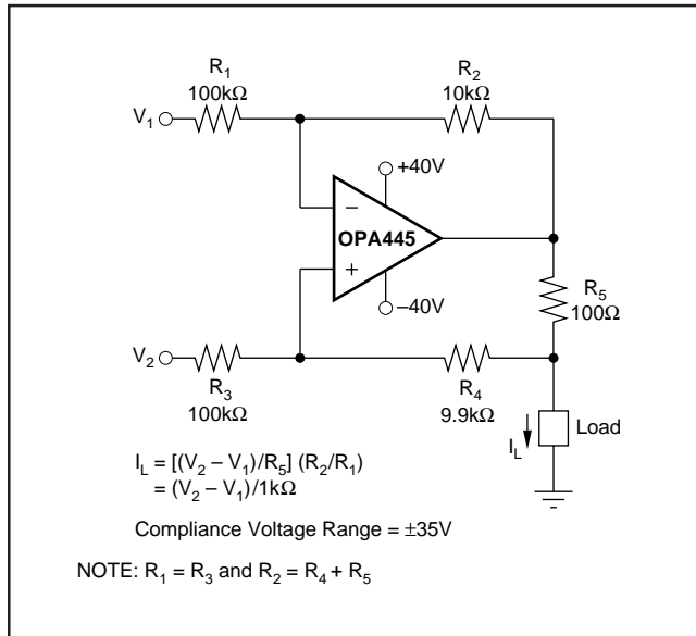
FIGURE 9. Voltage-to-Current Converter.
