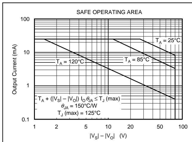
FIGURE 4. SO-8 Safe Operating Area.
