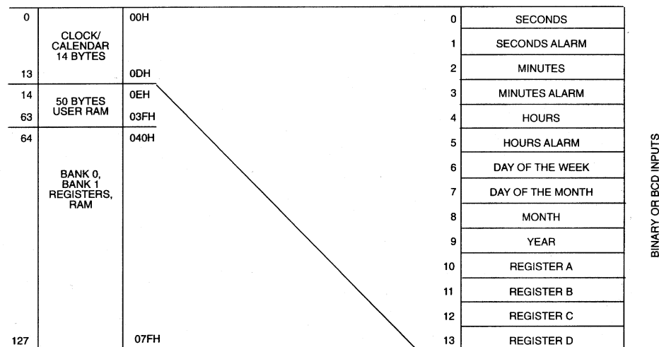
DS1689 REAL TIME CLOCK ADDRESS MAP Figure 2
