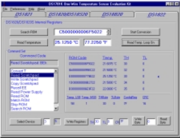
Figure 5.0 Resolution Selection
