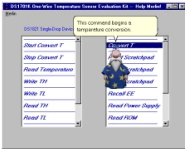
Figure 11.0 About Selection
