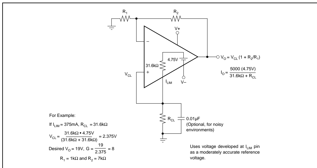
FIGURE 12. Voltage Source.
