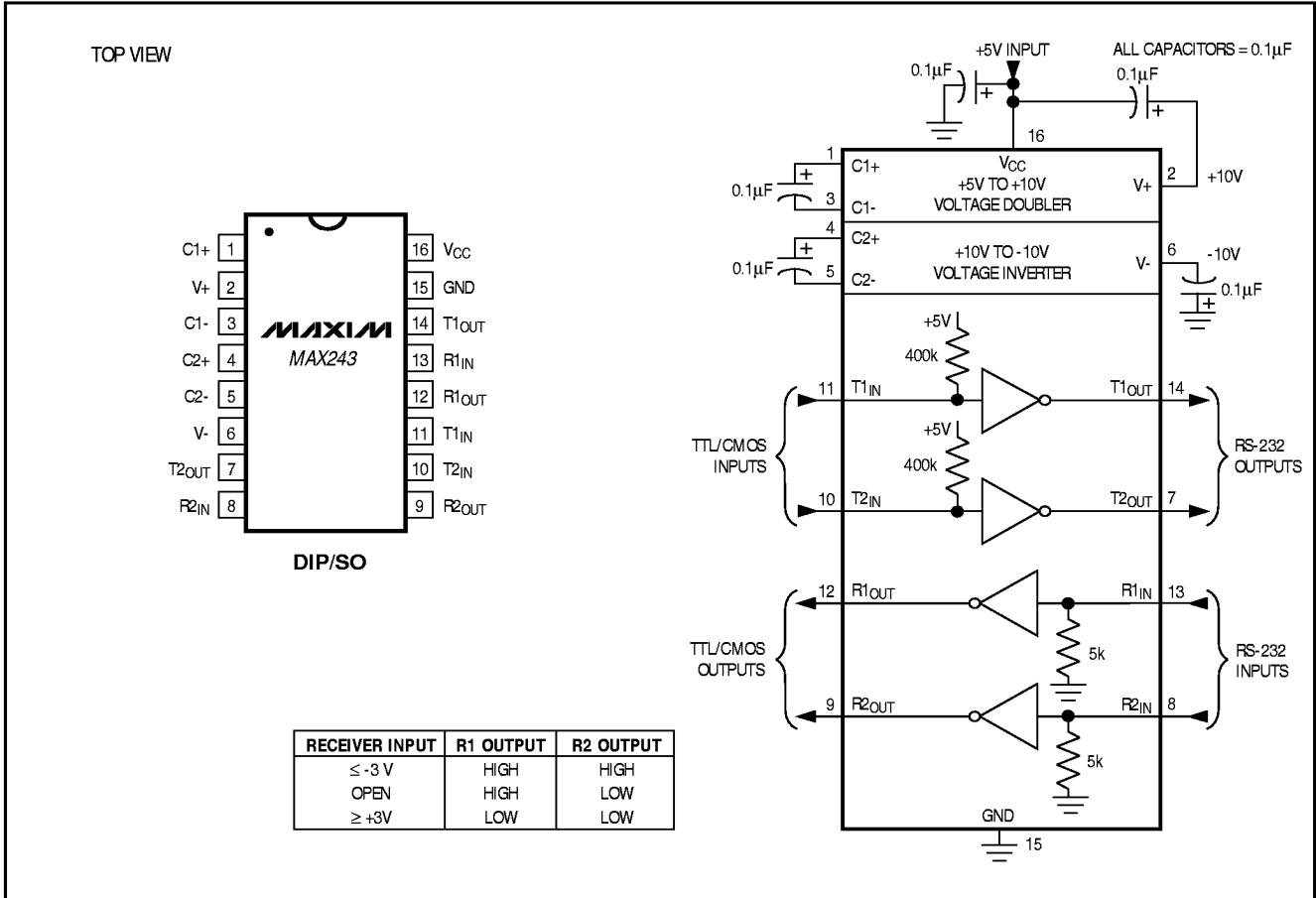
Figure 19. MAX243 Pin Configuration and Typical Operating Circuit
