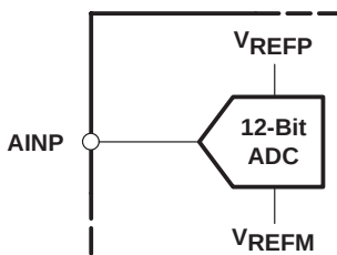
Figure 7. Single-Ended Input Stage
