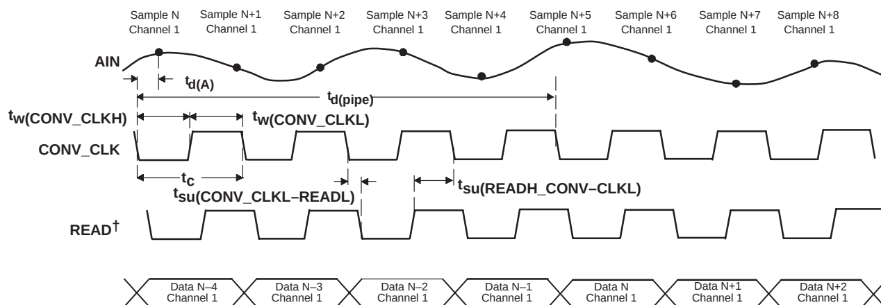
Figure 1. Conversion Timing in 1-Channel Operation
