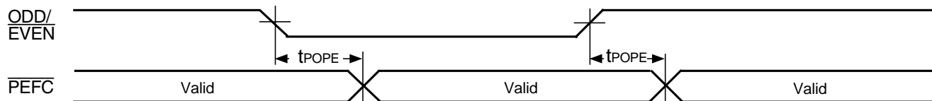
Figure 21. ODD/EVEN to \overline{PEFC} Timing
