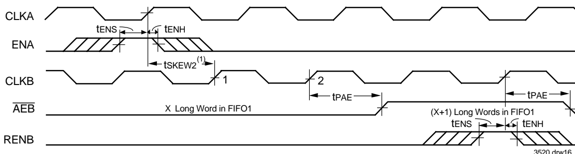
Figure 15. FFC Flag Timing and First Available Write when FIFO2 is Full
