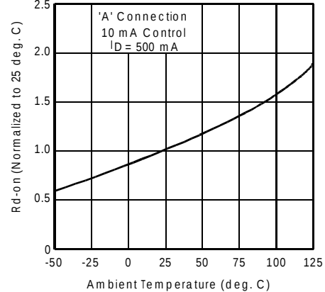
Figure 4. Typical Normalized On-Resistance
