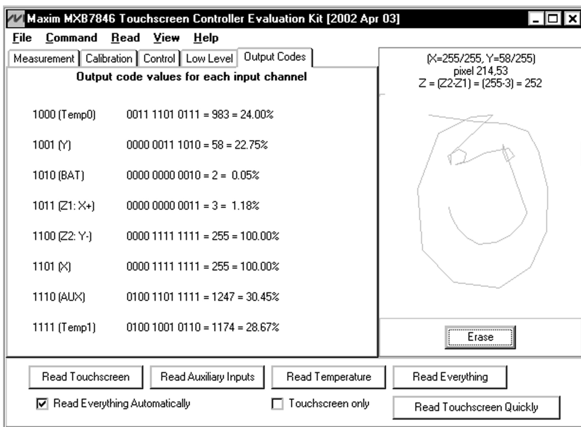
Figure 5. MXB7846 Touch-Screen Controller EV Kit—Output Codes
