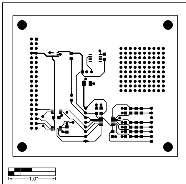
Figure 9. MXB7846 EV Kit PC Board Layout—Component Side
