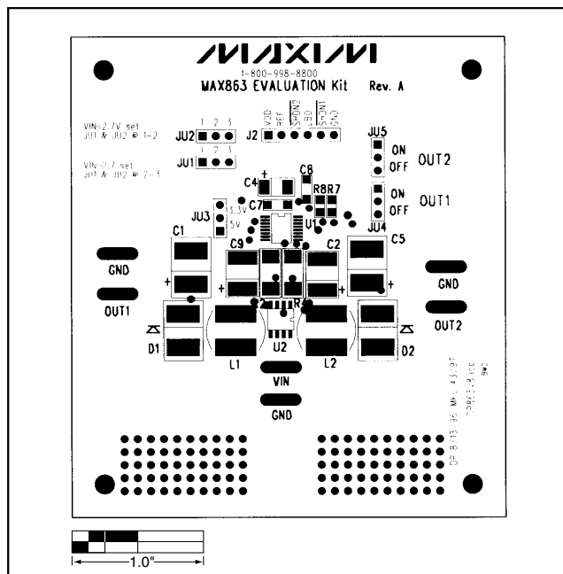
Figure 2. MAX863 EV Kit Component Placement Guide—Component Side
