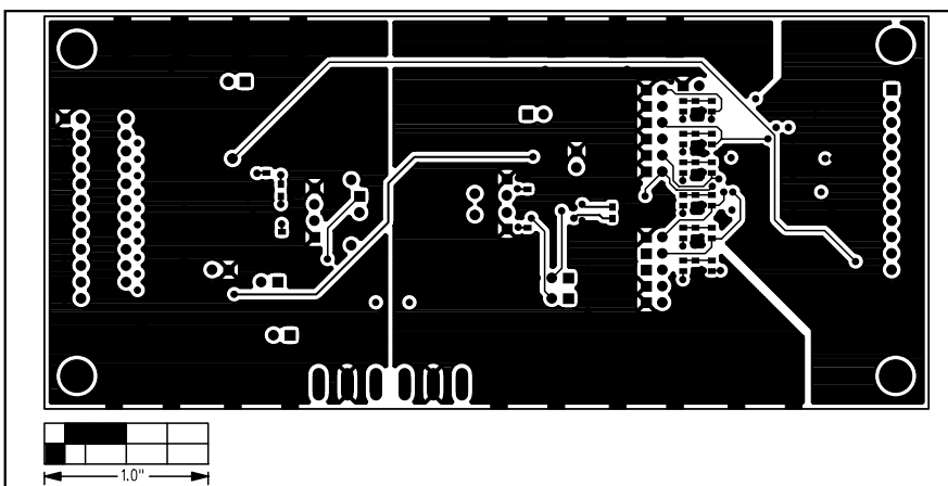
Figure 7. MAX9205 EV Kit PC Board Layout— Solder Side
