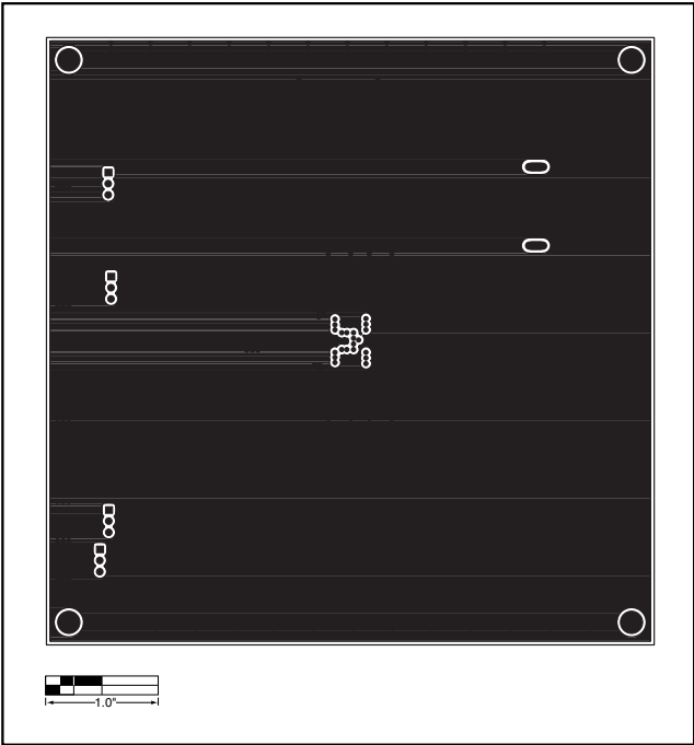
Figure 5. MAX9400 EV Kit PC Board Layout—Inner Layer 2 (GND Layer)
