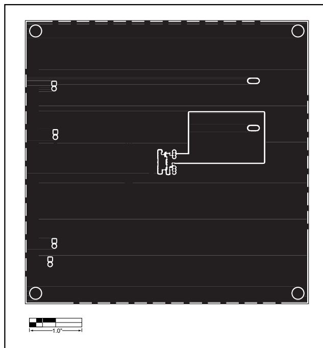
Figure 7. MAX9400 EV Kit PC Board Layout—Solder Side
