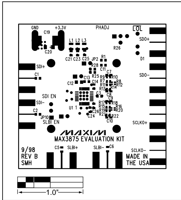
Figure 3. MAX3875 EV Kit Component Placement Guide
