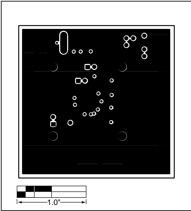
Figure 6. MAX3875 EV Kit PC Board Layout—Ground Plane
