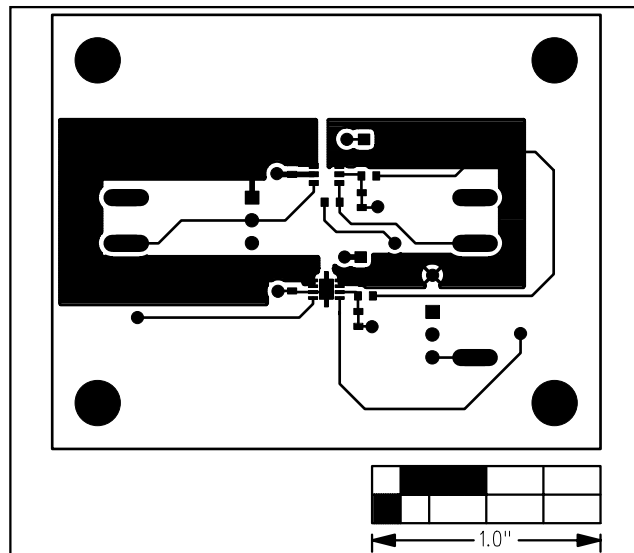
Figure 3. MAX6470 EV Kit PC Board Layout—Component Side
