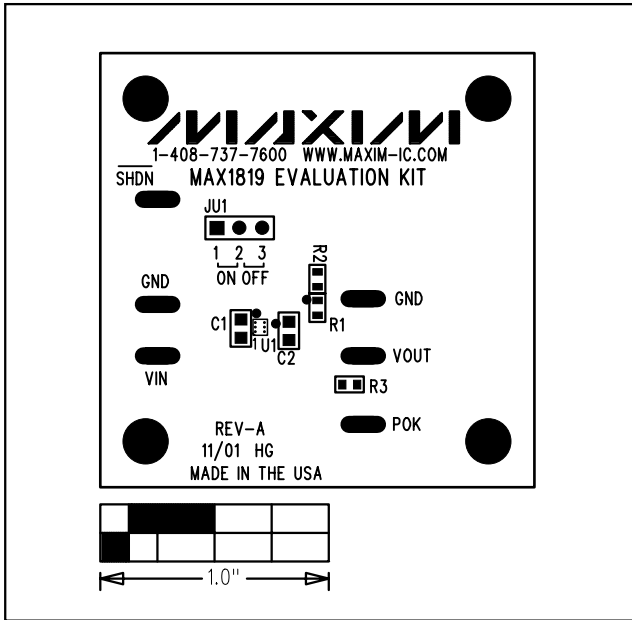
Figure 2. MAX1819 EV Kit Component Placement Guide—Component Side
