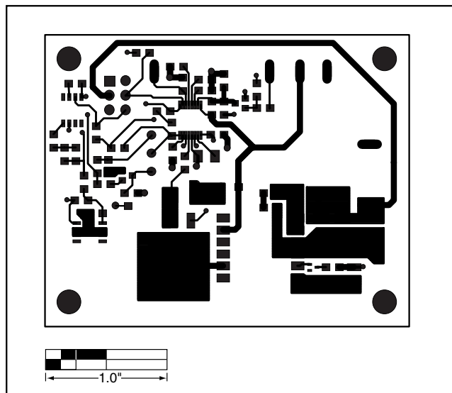
Figure 3. MAX5003 EV Kit PC Board Layout—Component Side
