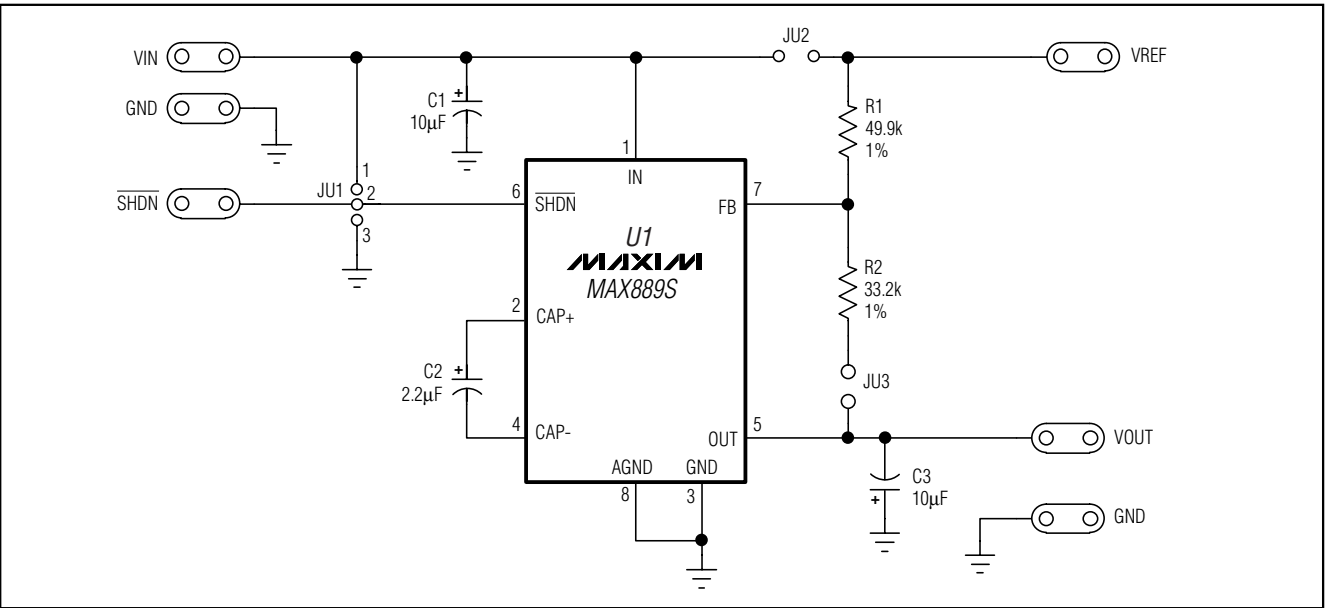
Figure 1. MAX889S EV Kit Schematic Diagram
