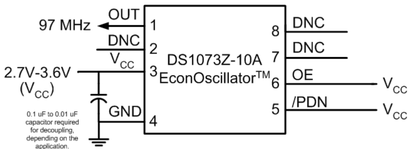
Figure 2. DS1073Z-10A Configuration
