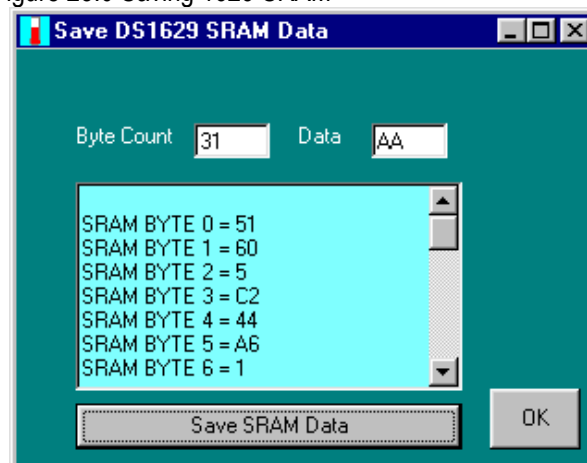
Figure 23.0 Saving 1629 SRAM
