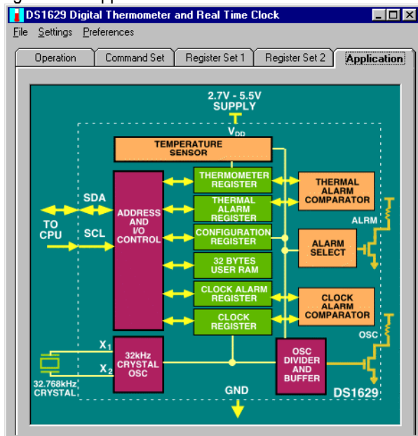
Figure 26.0 Application Tab
