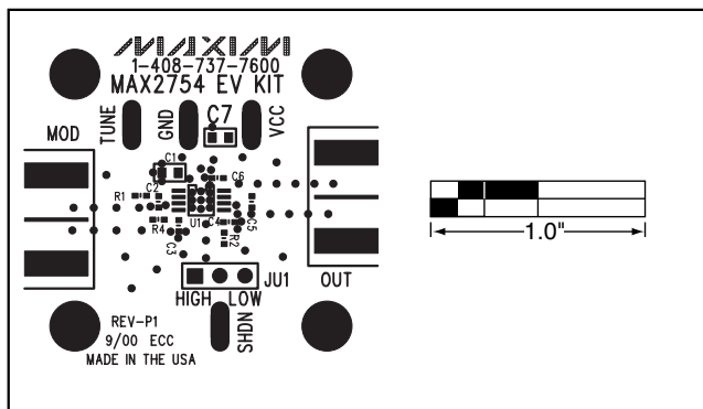
Figure 2. MAX2754 EV Kit Component Placement Guide—Top Silkscreen
