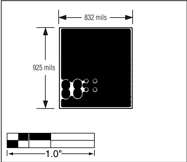
Figure 4. MAX2648 EV Kit PC Board Layout—Ground Plane
