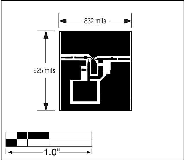
Figure 2. MAX2648 EV Kit PC Board Layout—Component Side
