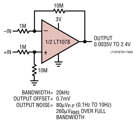
Gain of 10 Difference Amplifier
