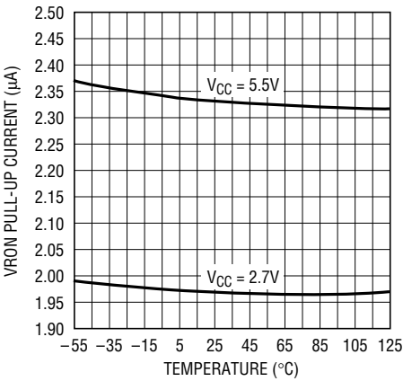
VRON Pull-Up Current vs Temperature
