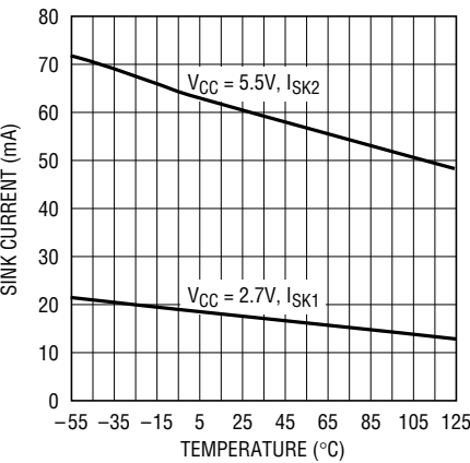
SDA, PGTMR, CPUON Sink Current vs Temperature
