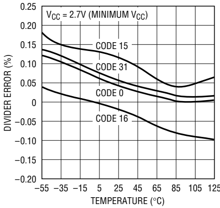
Resistor Divider Error vs Temperature
