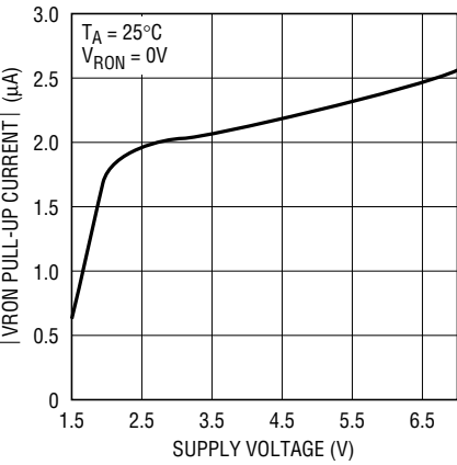
VRON Pull-Up Current vs Supply Voltage
